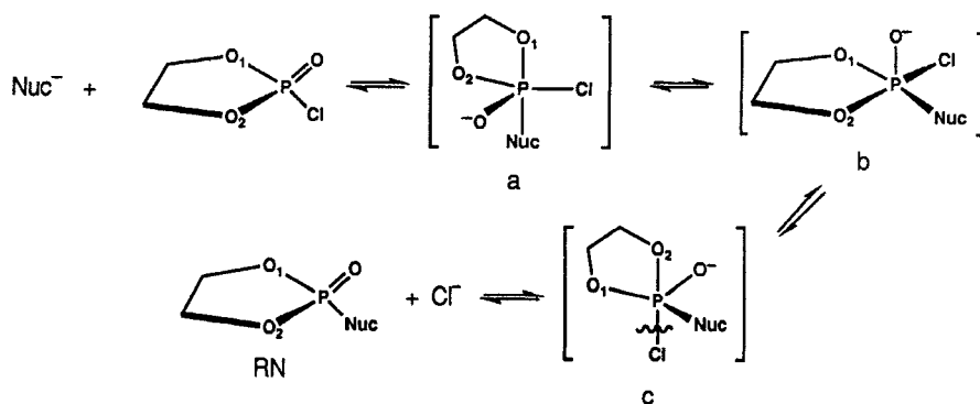
FIGURE 4 Reaction mechanism for a solvolysis reaction proceeding with pseudorotation according to the retention scheme in Figure 1b.
