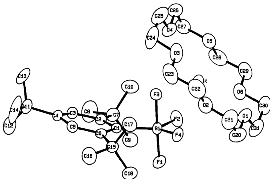
FIGURE 6 ORTEP plot of the cation-anion pair in [(t\text{-Bu})_3\text{C}_6\text{H}_2\text{SiF}_4][\text{K}, 18\text{-crown-6}] \cdot \text{CH}_2\text{Cl}_2 ( 24 ) with thermal ellipsoids at the 30% probability level. Hydrogen atoms are omitted for clarity.
