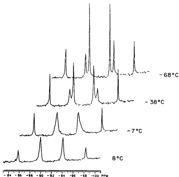
FIGURE 7 Variable-temperature 29 Si NMR spectra of [Mes 2 SiF 3 ][K,18-crown-6] showing retention of 29 Si— 19 F spin-spin coupling from the “stopped” exchange region, -68 °C, to the fast exchange region, 8 °C.
