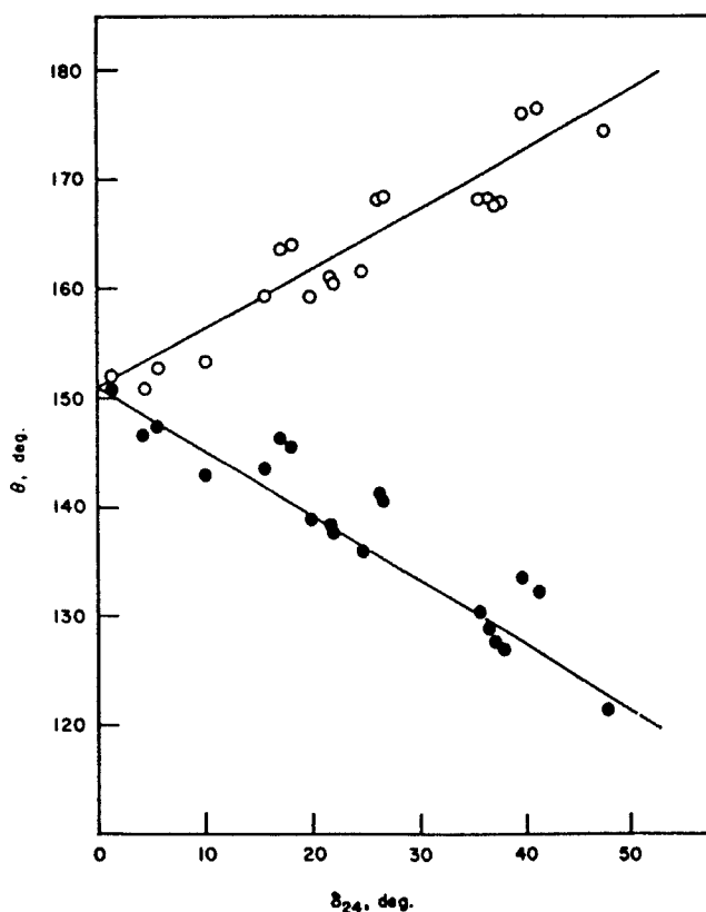
FIGURE 5 Variations of the axial angle, \theta_{15} (open circles), and equatorial angle, \theta_{24} (filled circles), vs the dihedral angle, \delta_{24} , as structural distortion for pentacoordinated silicon(IV) compounds listed in Table VII of ref 31 and in Table IV of ref 29 proceeds along the Berry coordinate from a rectangular pyramid toward a trigonal bipyramid. The least-squares lines \theta_{15} = 0.5697\delta_{24} + 150.0 and \theta_{24} = -0.5778\delta_{24} + 151.9 give an average value of 151.0^\circ for the trans basal angle of the "limiting" rectangular pyramid. The solid lines were determined by the values of 180 and 120^\circ for the ideal trigonal bipyramid, \delta_{24} = 53.1^\circ , and 151.0^\circ at \delta_{24} = 0^\circ .
