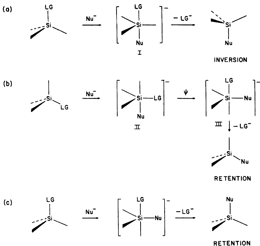
FIGURE 1 Mechanisms for nucleophilic substitution reactions of silicon: (a) inversion; (b) retention involving axial attack and pseudorotation to give axial departure; (c) retention involving equatorial attack and axial departure. \psi symbolizes a pseudorotational process.
